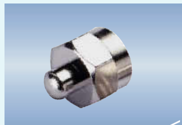
F-319A F MALE DUMMY LOAD 75 OHM (5-1500MHz RETURN LOSS -25dB)
